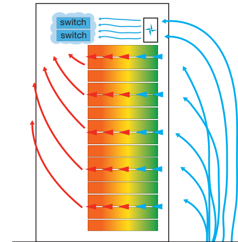
Opengate Switch Cooling guides cool air to network devices mounted in non-ideal locations within the cabinet. In many cases this can be done with a simple passive device. Active fans may be incorporated as configuration, size and airflow requirements demand.
